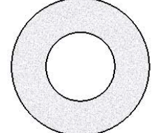
1.030 x .515 x .062 894860
